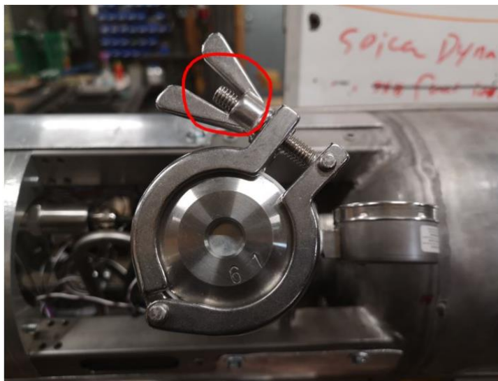
Figure 9: Nominal clamp position with one burst disc. (Source: Copenhagen Suborbitals)
