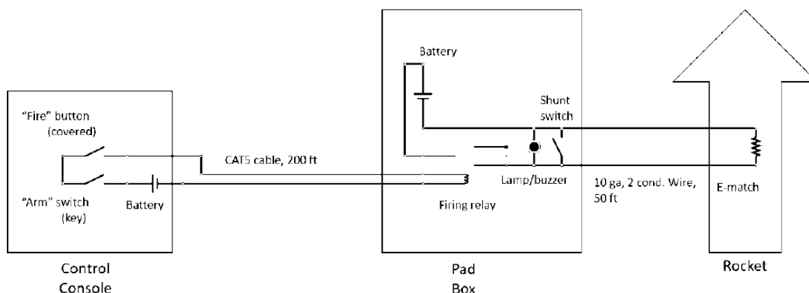
Figure 14: An improved high current fire control system.
