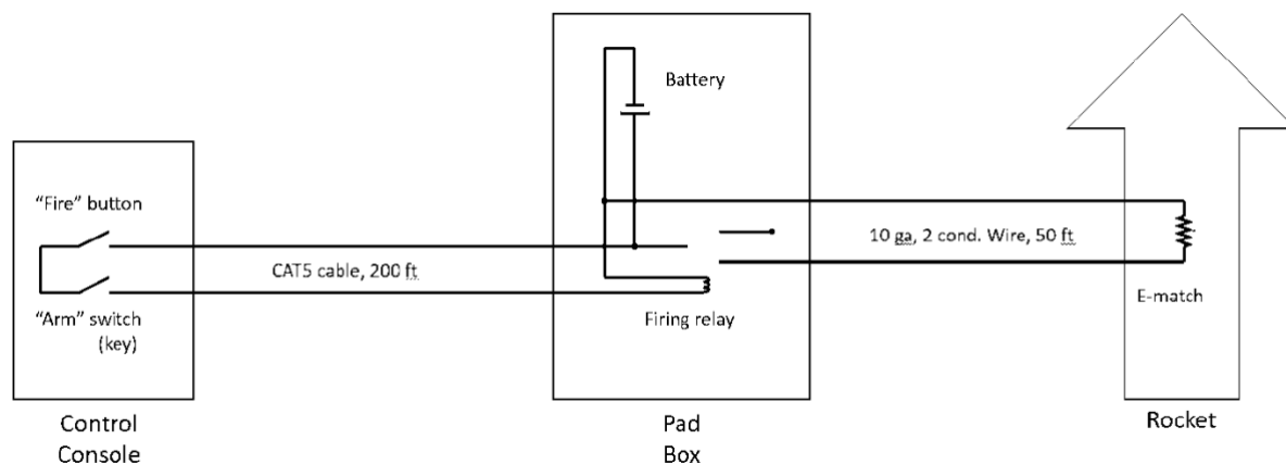
Figure 13: A simple high current fire control system.
